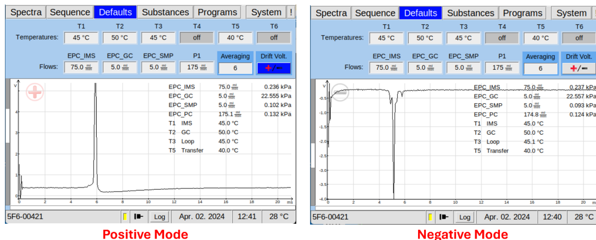
Figure 31: Drift Voltage Windows - positive and negative Mode
